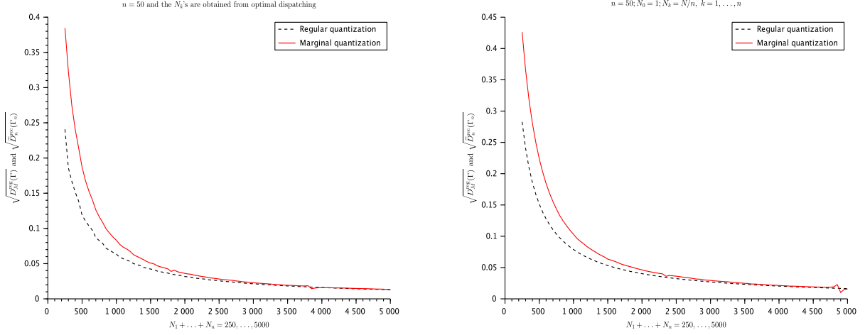
Figure 1: Comparison of the regular quantization (Regular quantization) of W_1 with its recursive marginal quantization (Marginal quantization) (where W is a Brownian motion). Abscissa axis: n = 50 and the total budget N = N_1 + \dots + N_n varies from 250 up to 5000. Ordinate axis: For a given N , (a) (left hand side graphic) we depict the recursive quantization errors (\tilde{D}_n^{\text{rec}}(\Gamma_n))^{1/2} where |\Gamma_n| is given by the optimal dispatching procedure, and the regular quantization errors (D_M^{\text{reg}}(\Gamma))^{1/2} for M = |\Gamma_n| ; (b) (right hand side graphics) we set N_k = N/n , for k = 1, \dots, n and depict the recursive quantization errors (\tilde{D}_n^{\text{rec}}(\Gamma_n))^{1/2} , for |\Gamma_n| = 5, \dots, 100 , and the regular quantization errors (D_M^{\text{reg}}(\Gamma))^{1/2} , for M = |\Gamma| = 5, \dots, 100 .
