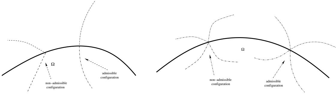
Non-admissible and admissible configurations (a) one vortex (b) two vortices.
