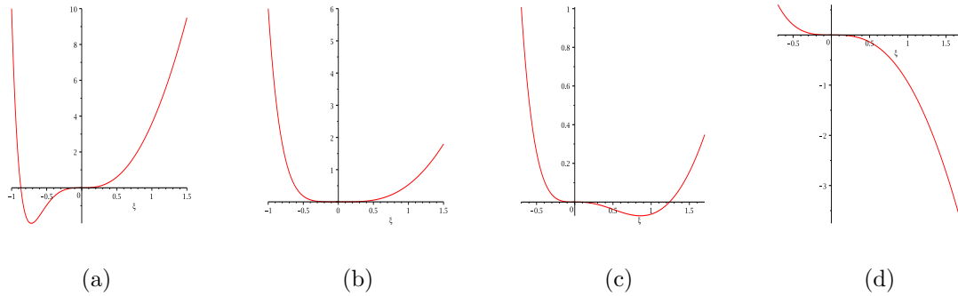
Figure 35: Graphs of \mathcal{V} for (a) \varrho_0 = 0.2 ; (b) \varrho_0 = 1/3 ; (c) \varrho_0 = 0.4 ; (d) \varrho_0 = 1
