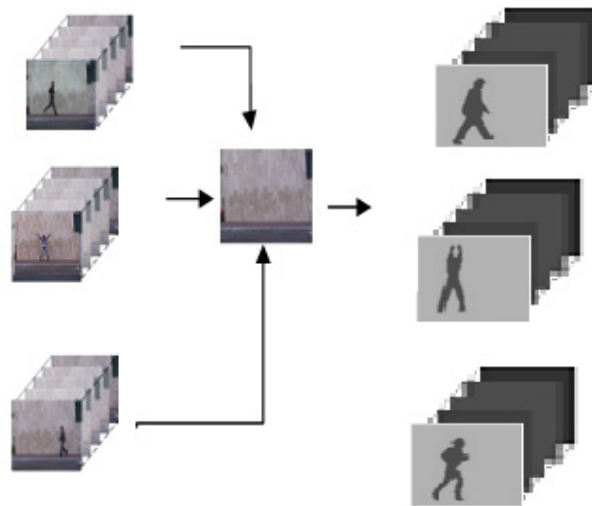
Fig. 2. Background subtraction
