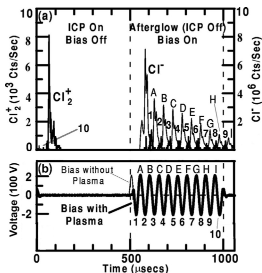
FIG. 10. Mass spectrometer signals for (a) Cl + and Cl - , and (b) applied bias voltage measured in a 1 mTorr, 5 sccm Cl 2 ICP plasma with a peak ICP power of 600 W pulsed at 1 kHz and 50% duty cycle. The bias operates at an excitation frequency of 20 kHz with a peak voltage of 225 V. Reprinted with permission from S. K. Kanakasabapathy, L. J. Overzet, V. Midha, and D. Economou, Appl. Phys. Lett. 78 , 22 (2001). Copyright 2001, American Institute of Physics.
