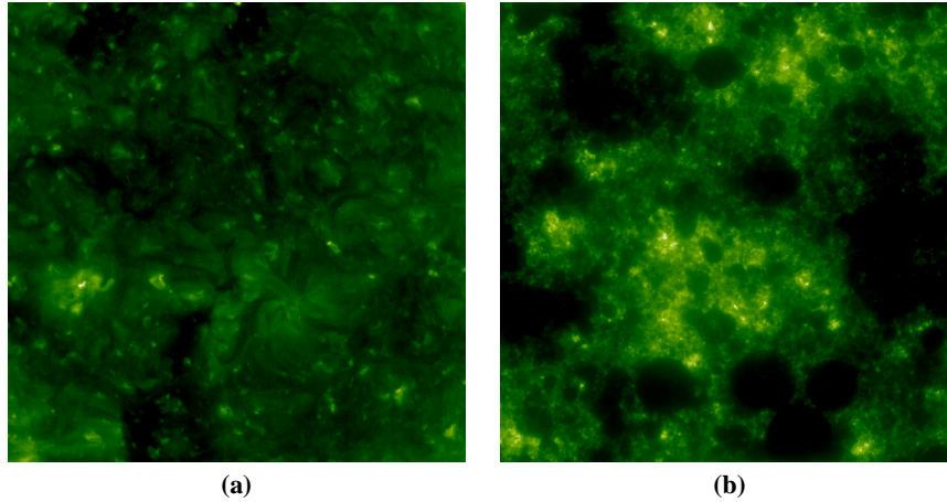
Fig. 5. Examples of 512 \times 512 images of (a) Quiet Sun, (b) a fractionally integrated compound Poisson cascade.
