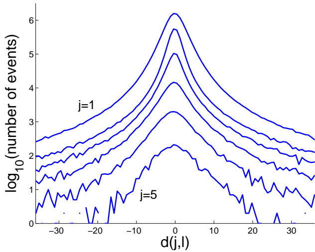
Fig. 3. Histograms of 2-D discrete wavelet coefficients computed from 54 Quiet Sun images taken by EIT at 19.5 nm during the year 1997.
