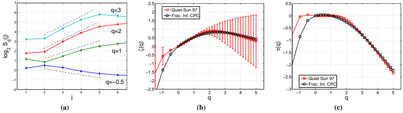
Fig. 4. (a) Structure function ( q = -0.5, 1, 2, and 3 ) estimated from DWT of Quiet Sun images in 1997. (b) Exponents \zeta(q) obtained from the DWT structure functions, for the original Quiet Sun images, and for simulated images using Compound Poisson Cascades (c) Exponents \tau(q) deduced from \zeta(q) by \tau(q) = \zeta(q) - q\zeta(1) .
