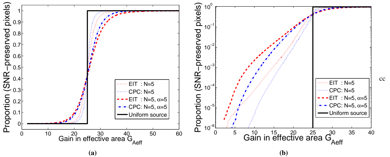
Fig. 6. Simulation of the proportion of pixels in an HRI instrument at perihelion that will conserve the same SNR as in the case of EIT at L1 (we term these “SNR-preserved pixels”) given a factor of increase of the effective area in (a) linear and (b) semi-logarithmic representation. Both EIT data (Real) and synthetic data (CPC) are represented in case of 1) a better angular resolution ( N=5 ), 2) a better angular resolution and a smaller distance ( N=5, \alpha=5 ). For a gain in effective area equal to 15, 1.6% of the pixels are SNR-preserved on real EIT data when N=5, \alpha=5 . This figure becomes 0.2% when G_{Aeff}=10 only.
