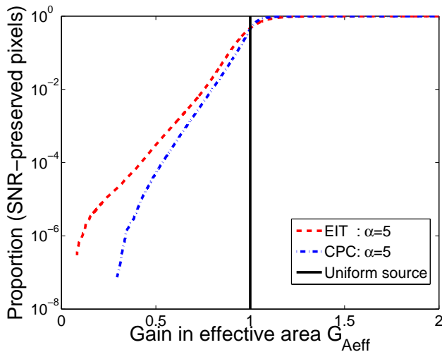
Fig. 7. Proportion of pixels having a similar SNR at low resolution (far from the Sun) and at high resolution ( \alpha=5 times closer to the Sun) for a given change in effective area. When getting closer to the Sun, one may have a reduced effective area and still have a proportion of pixels with preserved SNR.
