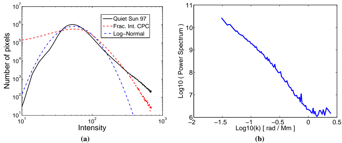
Fig. 2. (a) Histogram of original data set in log-log scale, together with a lognormal distribution having the same mean and variance, and the histogram of a set of 54 artificial images generated by a multiplicative cascade model. (b) Omnidirectional power spectrum. For Fourier wavenumbers 0.03 < ||k|| < 1.12 rad/Mm, the spectrum exhibits a power law with index equal to -2.8 (estimation using least squares).
