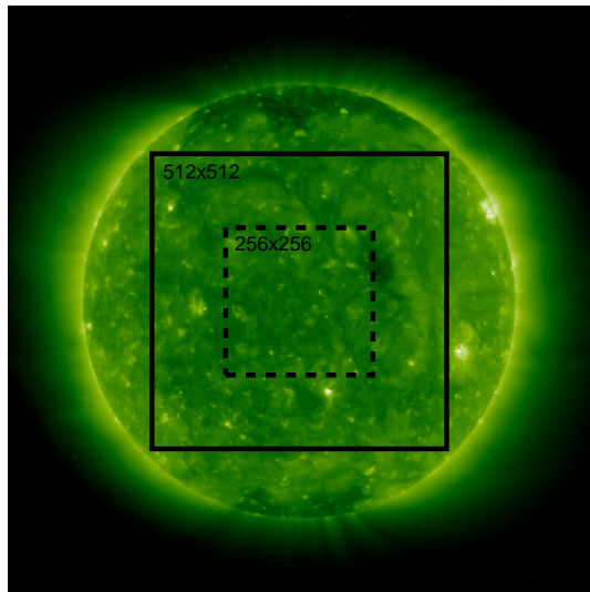
Fig. 1. Example of a Quiet Sun images seen by EIT in 19.5 nm, with indication of the squared area taken into account. The multifractal analysis characterizes the region within the square of size 256 \times 256 .
