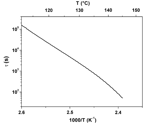
Fig. 7. Arrhenius plot of relaxation times associated with \alpha relaxation process recorded with TSDC measurements.
