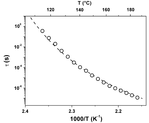
Fig. 6. Arrhenius plot of relaxation times associated with \alpha relaxation process recorded with DDS measurements.
