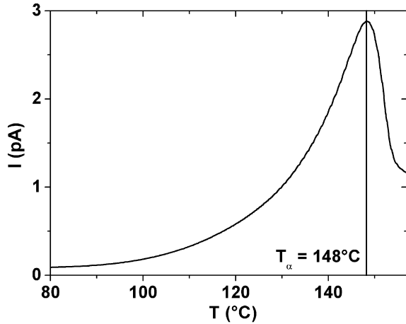
Fig. 5. TSDC complex spectrum of PC sample recorded after a polarisation at T_p = 155 °C for 2 min with E = 0.4 MV m -1 .
