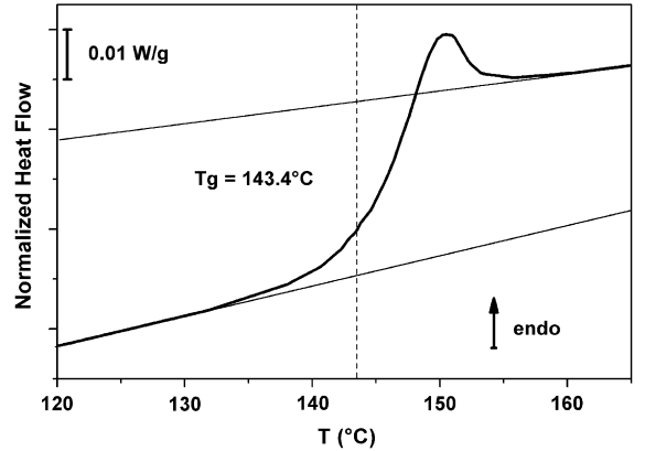
Fig. 3. DSC measurements of PC sample after a cooling from 180\text{ }^\circ\text{C} to 60\text{ }^\circ\text{C} with cooling rates q_c = 10\text{ }^\circ\text{C}/\text{min} and q_h = 10\text{ }^\circ\text{C}/\text{min} .
