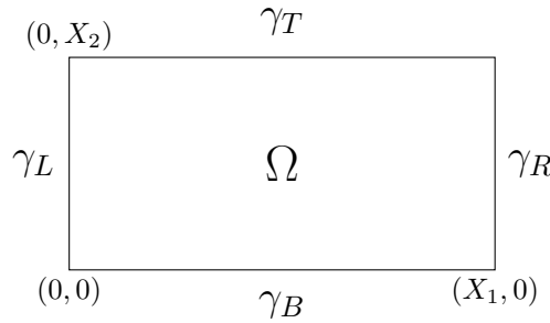
Figure 1: Domain \Omega for section 2.5.
