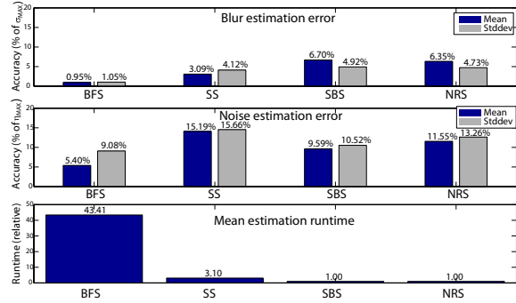
Figure 4. Performance and accuracy comparison of four search algorithms.
