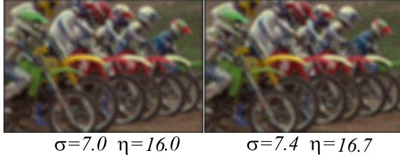
Figure 3. Typical result obtained by a search strategy. Given an image f (here Bikes ) and a degraded image g whose degradation parameters are (7.0, 16.0) , the recovered parameters (7.4, 16.7) give a new figure \hat{g} (on the right) that is very similar to g (on the left).
