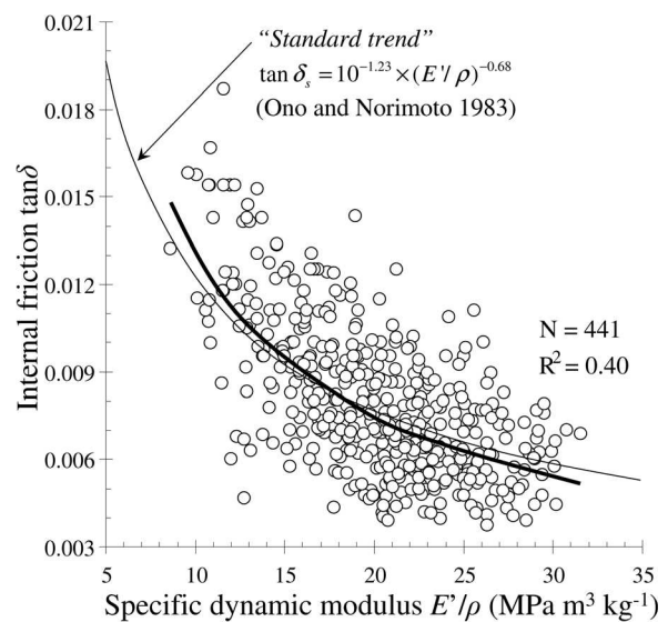
FIG. 4. Relation between the average damping coefficient (or internal friction, \tan\delta ) and the average specific dynamic modulus of elasticity ( E'/\rho ) for 441 species.
