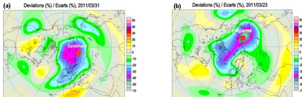
Fig. 6. WOUDC total ozone mapping on 23 and 31 March 2011 when the low ozone vortex passed over Salekhard (a) and Zhigansk (b) . The initial plots of the total ozone deviation are from the WOUDC database http://www.woudc.org/data_e.html .
