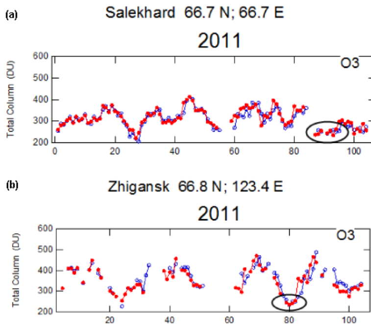
Fig. 4. SAOZ spectrometerr total ozone real-time data at the Salekhard aerological station (a) and at the Zhigansk aerological station (b) in January–April 2011. The initial plots are from the World SAOZ real time database http://saoz.obs.uvsq.fr/SAOZ-RT.html .
