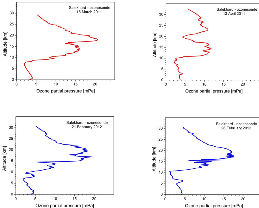
Fig. 7. Ozone profiles from 2Z-ECC sondes in Salekhard in the polar vortex in March–April 2011 (red) and in February 2012 (blue).
