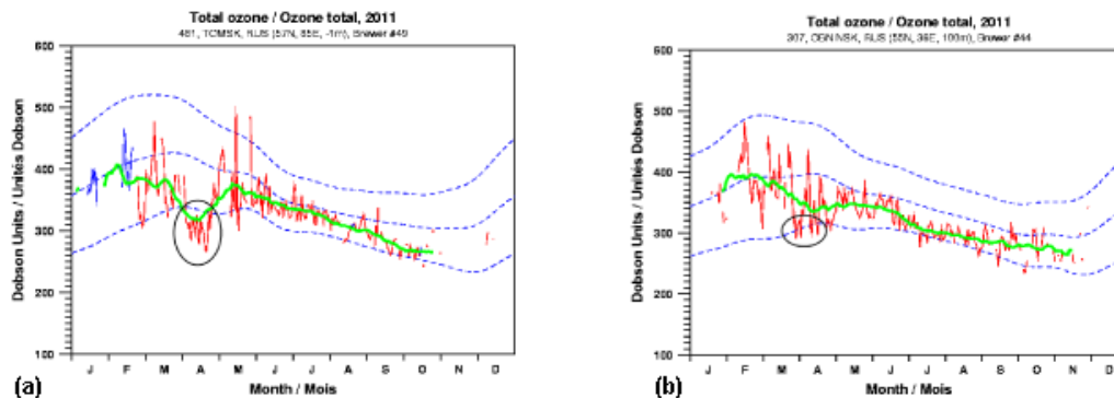
Fig. 3. The result of the Brewer MKIV No 049 total ozone measurements in Tomsk in 2011 (a) and the Brewer MKII No 044 total ozone measurements in Obninsk in 2011 (b) . The initial plots are from the WOUDC database http://www.woudc.org/data.e.html .
