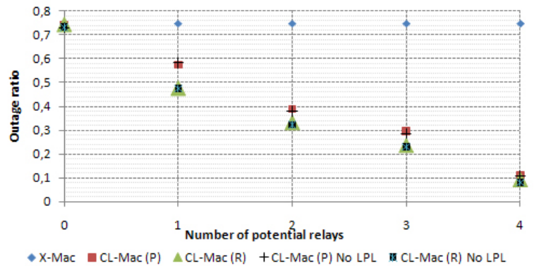
Fig. 4. Outage Ratio Vs Potential Relays
