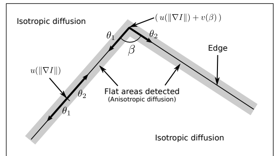
Figure 1: Control functions (u, v) and diagram of our diffusion scheme.
