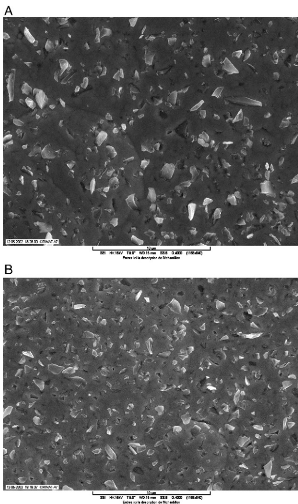
Fig. 6. Micrographs obtained by SEM of the composite coatings: A) 120 g L -1 SiC and 3.5 · 10 -4 M CTAHS; B) 200 g L -1 SiC and 3.5 · 10 -4 M CTAHS.
