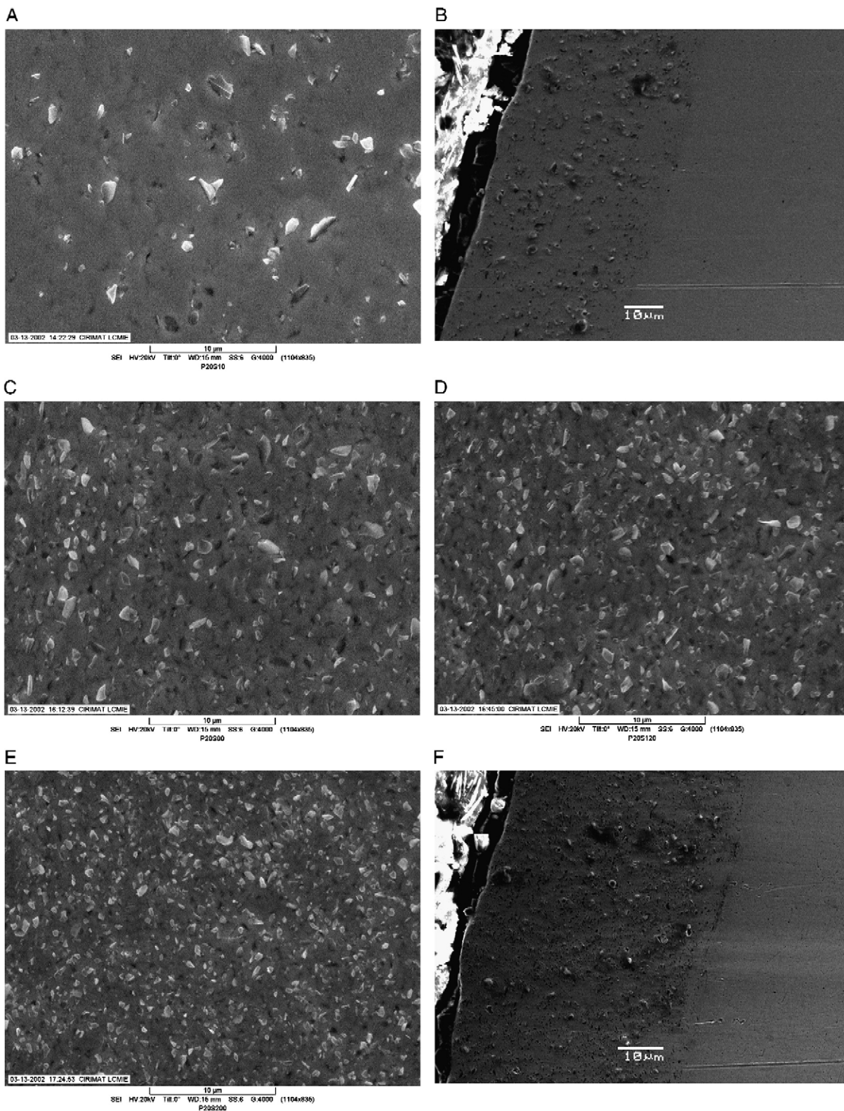
Fig. 2. SEM micrographs of composite NiP-SiC coating obtained from bath with different concentration of SiC particles ( 20 \text{ g L}^{-1} \text{ H}_3\text{PO}_3 in electrolyte): A) 10 \text{ g L}^{-1} SiC; B) 10 \text{ g L}^{-1} SiC (cross-section); C) 80 \text{ g L}^{-1} SiC; D) 120 \text{ g L}^{-1} SiC; E) 200 \text{ g L}^{-1} SiC; F) 200 \text{ g L}^{-1} SiC (cross-section).
