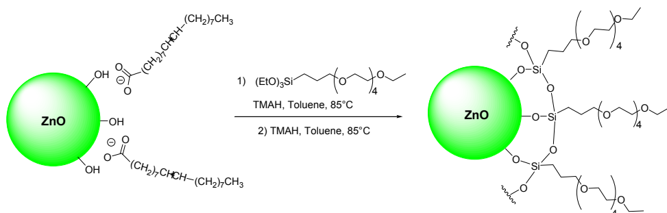
Fig. 10. Synthesis of PEG-siloxane capped ZnO quantum dots.
