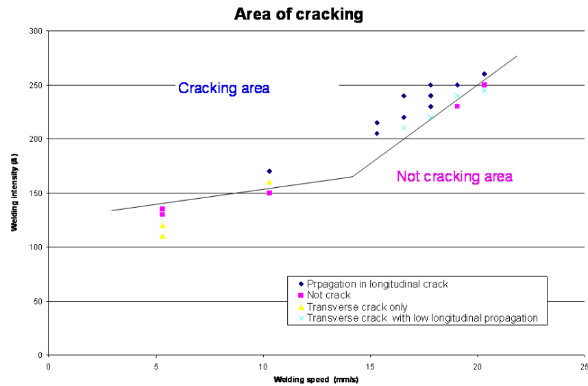
Figure 6: Hot cracking area
