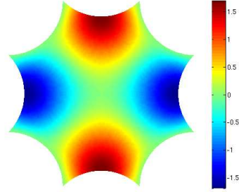
(c) Symmetry \mathbf{D}_2 = \langle -Id, \kappa \rangle .
