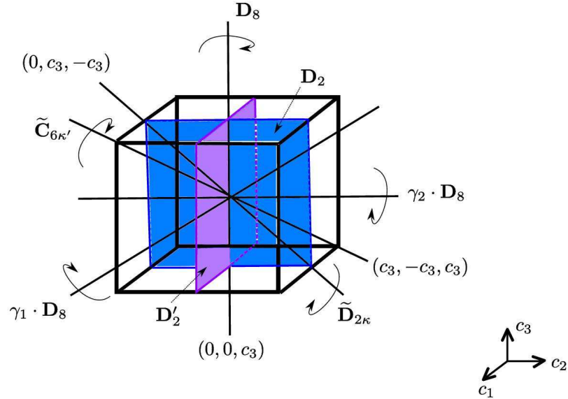
FIGURE 6. Maximal isotropy subgroups \mathbf{D}_8 , \tilde{\mathbf{C}}_{6\kappa'} and \tilde{\mathbf{D}}_{2\kappa} of \mathbb{O} \rtimes \mathbb{Z}_2 . The axes \gamma_1 \cdot \mathbf{D}_8 and \gamma_2 \cdot \mathbf{D}_8 are copies of \mathbf{D}_8 by the elements \gamma_1, \gamma_2 \in \mathcal{G} (see 4.2.3). The plane (0, c_2, c_3) (resp. (c_1, 0, c_3) ) has symmetry \mathbf{D}_2 (resp. \mathbf{D}_2' ).
