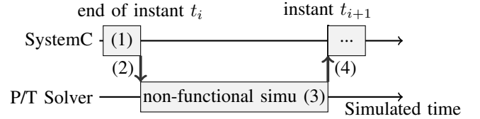
Fig. 6. lockstep cosimulation strategy. For clarity, simulated instants are represented with a non-null width.
