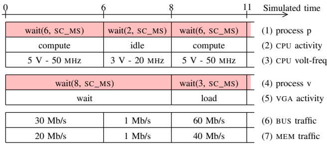
Fig. 3. Power Parameter Trace of the Example in Section III
