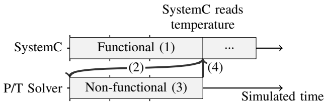
Fig. 8. functional ahead strategy, in the absence of interrupt
