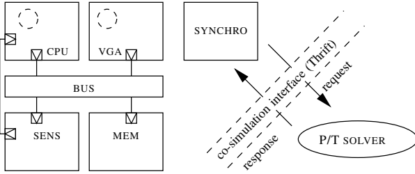
Fig. 5. Architectural View of the Cosimulation
