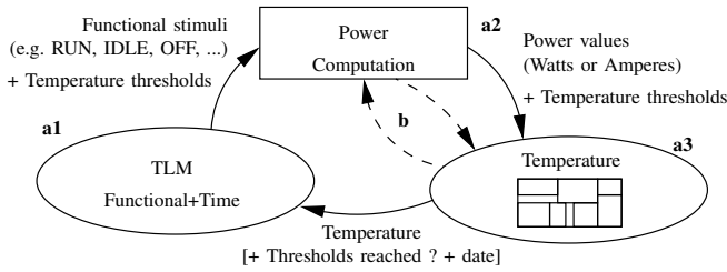
Fig. 1. a1, a2, a3 : one step of the co-simulation principle, b : temperature/power consumption feedback effect
