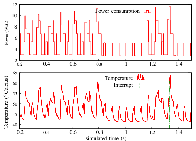
Fig. 9. Power and thermal simulation for the case study of section III
