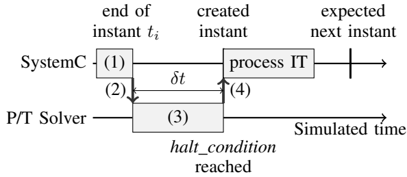
Fig. 7. lockstep cosimulation strategy with interrupt
