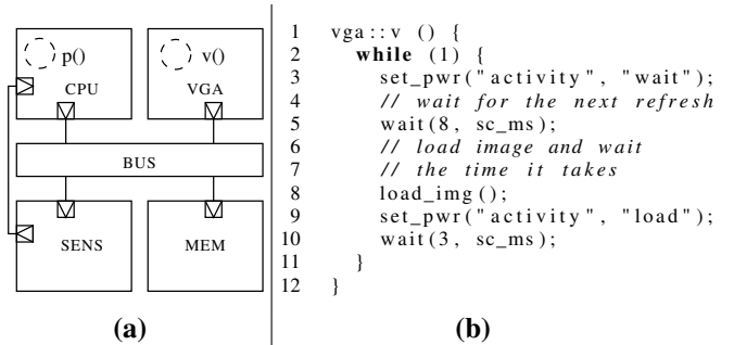
Fig. 2. Example TLM model and SystemC code of the threads
