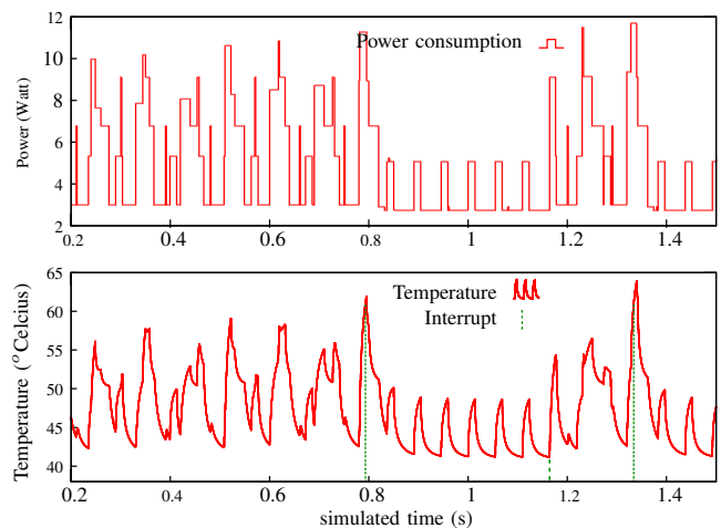
Fig. 9. Power and thermal simulation for the case study of section III
