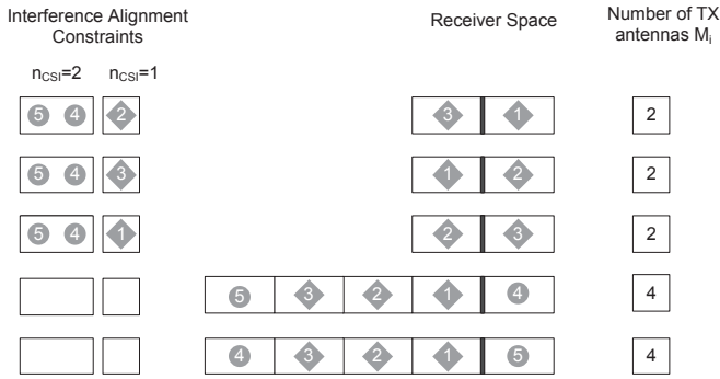
Fig. 1. Symbolic representation of the IA algorithm with incomplete CSIT for the tightly-feasible IC (2, 2).(2, 2).(2, 2).(4, 5).(4, 5) .
