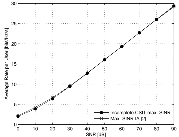
Fig. 2. Average rate per user in terms of the SNR for the tightly-feasible IC (2, 2).(2, 2).(3, 3).(3, 3).(5, 5).(6, 6).(7, 7) .
