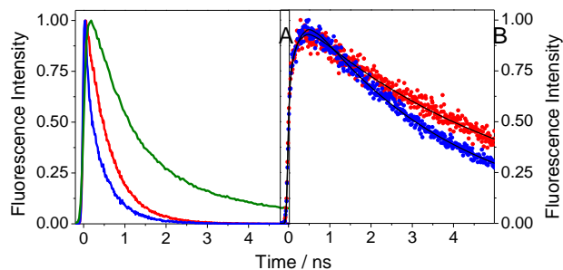
Figure 2. Normalised TCSPC decay traces at A) ( \lambda_{\text{em}} = 340 \text{ nm} ), B) ( \lambda_{\text{em}} = 450 \text{ nm} ) of ( S )-TrpMe (green), ( S,S )-FBP-TrpMe (red) and ( R,S )-FBP-TrpMe (blue). Fitted curves are shown in black.
