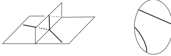
Figure 3: A r-embedding
