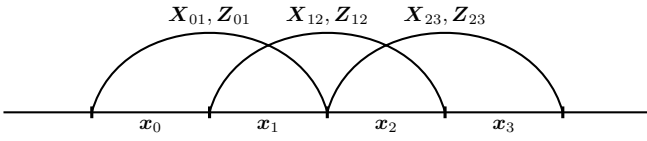
Fig. 2. Overlap and add in the time domain and corresponding TF-domain vectors. The time vectors \mathbf{x}_0, \mathbf{x}_1, \mathbf{x}_2 and \mathbf{x}_3 all have the same size M .
