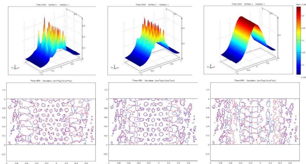
Fig. 6. Coincidence of the null-curvature lines of the u (in red) and v (in blue) concentration surfaces, when D_u/D_v varies from 0.05 (left) to 0.07 (right). For D_u/D_v = 0.06 (middle), the coincidence is perfect on the central part of the picture, which corresponds roughly to the experimental value of the diffusion coefficients ratio
