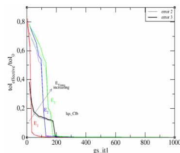
Figure 14: estimation of the effective tolerance artificially imposed for the Elastic_Repell_CLB law
