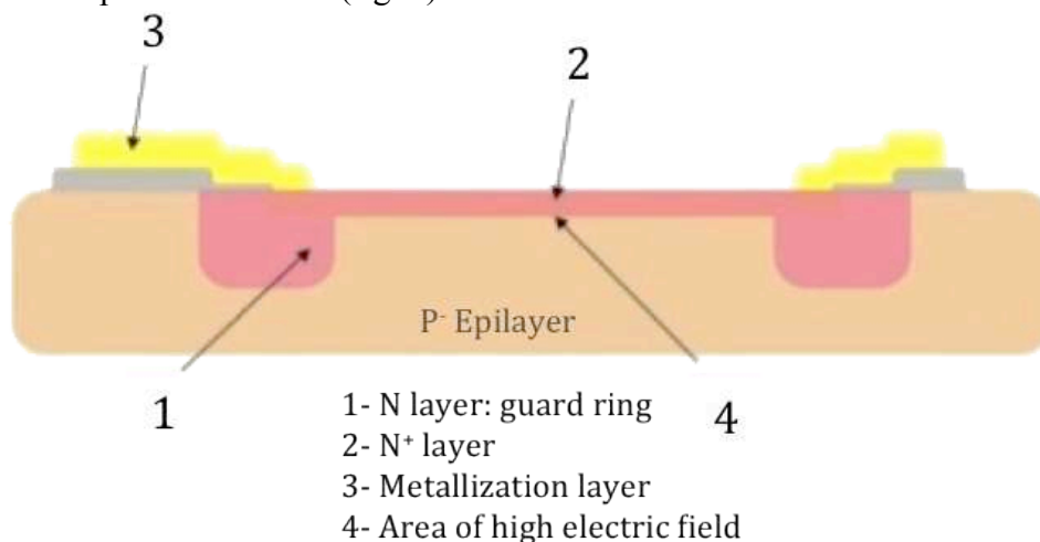
Figure 1: Geiger Photodiode structure based on N + /P junction and guard ring N layer.
