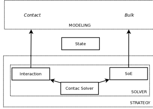
Figure 1. Rough architecture of LMGC90.
