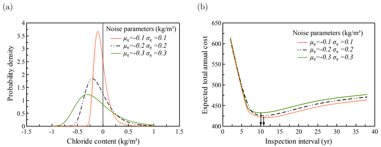
Figure 9: Influence of the quality of the inspection technique on the total expected annual costs.
