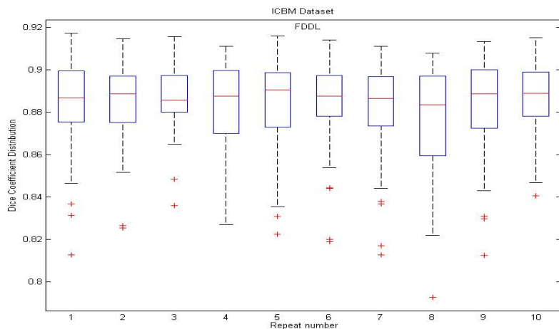
Figure 8: The performance of Fixed Discriminative Dictionary Learning on 80 ICBM subjects. The results were obtained by using a patch size of 5 \times 5 \times 5 voxels and a search volume of 7 \times 7 \times 7 voxels. The experiment was repeated 10 times. The average median Dice coefficient is 0.887.
