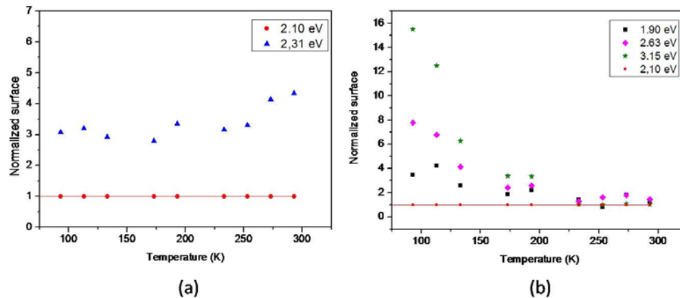
Fig. 4. Normalized surface of each luminescence band as a function of temperature for laser damage on silica materials. (a) 2.10 eV and 2.31 eV band. (b) 1.90, 2.63 and 3.15 eV band.
