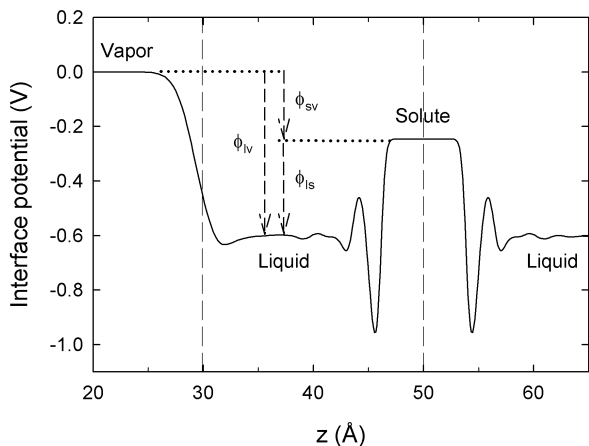
FIG. 1: Electric potential variation, \delta\phi(z) , across the vapor-liquid and the liquid-solute interfaces for the neutral LJ solute \Gamma^0 immersed in liquid water (SPC/E), at z = 50 Å. The Gibbs dividing surface (GDS) of the macroscopic interface and the solute position are indicated by dashed vertical lines.
