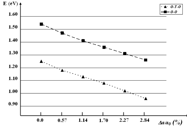
Figure 4. Octahedral–tetrahedral and octahedral–octahedral activation energy variations with the linear thermal expansion a .
