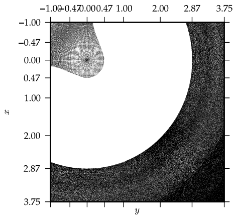
Figure 4.7.: Non-convexity region of the function f_{\text{test}}^2 on the domain [-1, 3.75]^2 computed through the smdDLFT; the points where the computed convex hull differs from the function f_{\text{test}}^2 are shown in white.
