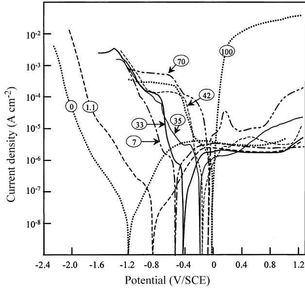
Fig. 3. Potentiodynamic polarization curves of different Al-Cu alloys in 0.1 M \text{Na}_2\text{SO}_4 solution (potential scan rate: 1 V/h). The number on each curve represents the atomic percentage of copper in the alloy.
