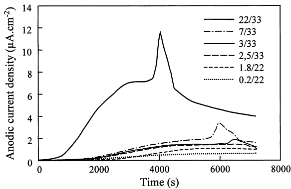
Fig. 8. Variation of anodic current density, i_a , with time for galvanic couples of Al-Cu alloys with copper content from 0.2 to 33 at.% Cu.
