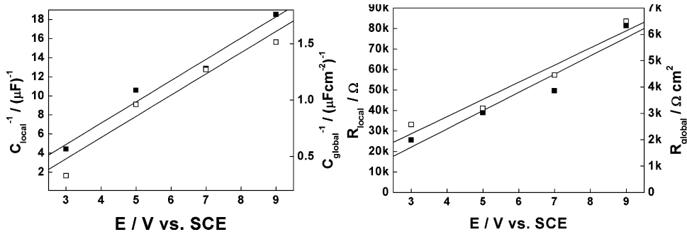
Fig. 7. High-frequency capacitance (left) and parallel resistance (right) as depending on potential calculated from the impedance spectra shown in Figs. 3 and 4.
