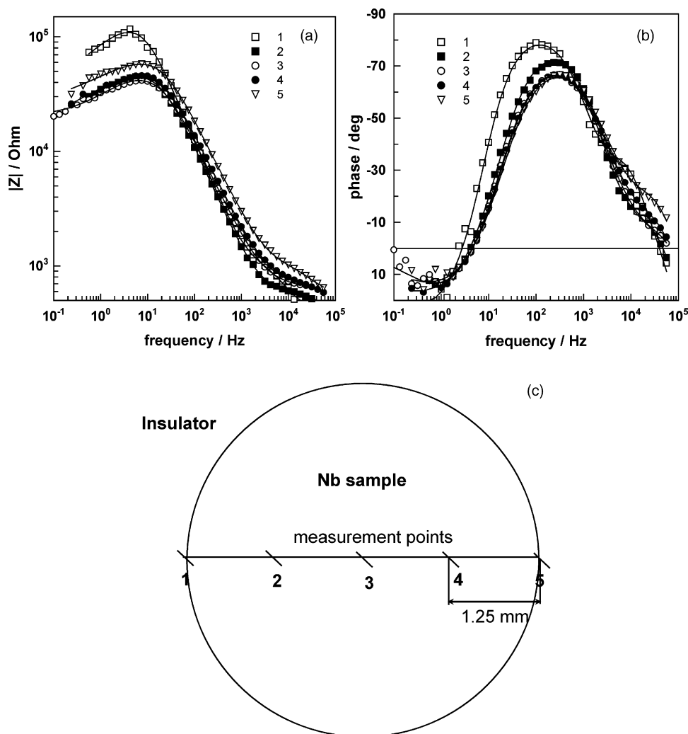
Fig. 5. Local impedance spectra for Nb oxidised at 5 V for 1 h (a: impedance magnitude vs. frequency; b: phase angle vs. frequency) at different points of the electrode surface, as indicated (c). Total diameter of the sample, 5 mm.
