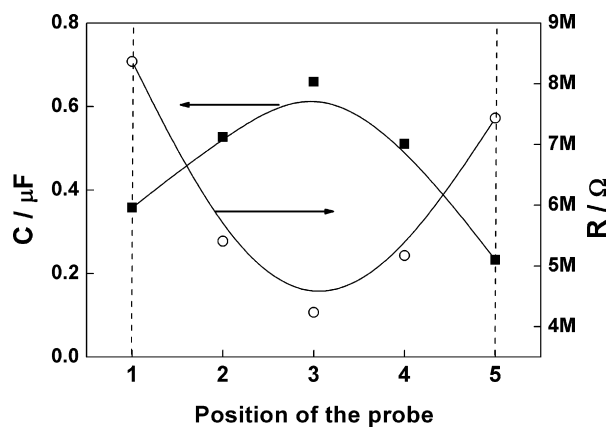
Fig. 11. Dependence of the capacitance and parallel resistance calculated from the spectra shown in Fig. 10 on the position of the LEIS probe.
