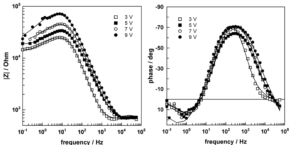
Fig. 4. Local impedance spectra at the centre of the electrode in conditions similar to those in Fig. 3.
