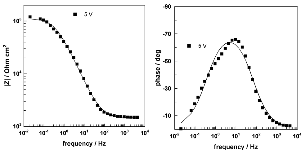
Fig. 9. Global impedance spectrum of a film formed in 1 M \text{H}_2\text{SO}_4 + 0.2\% HF for 1 h at 5 V and measured at the same potential in a 0.001 M \text{Na}_2\text{SO}_4 solution.
