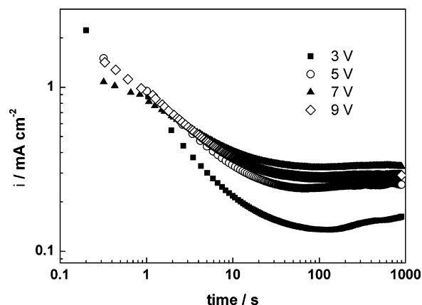
Fig. 2. Current density vs. time curves for Nb in 0.001 M \text{Na}_2\text{SO}_4 + 0.2% HF as depending on oxidation potential. Oxidation time 1 h.
