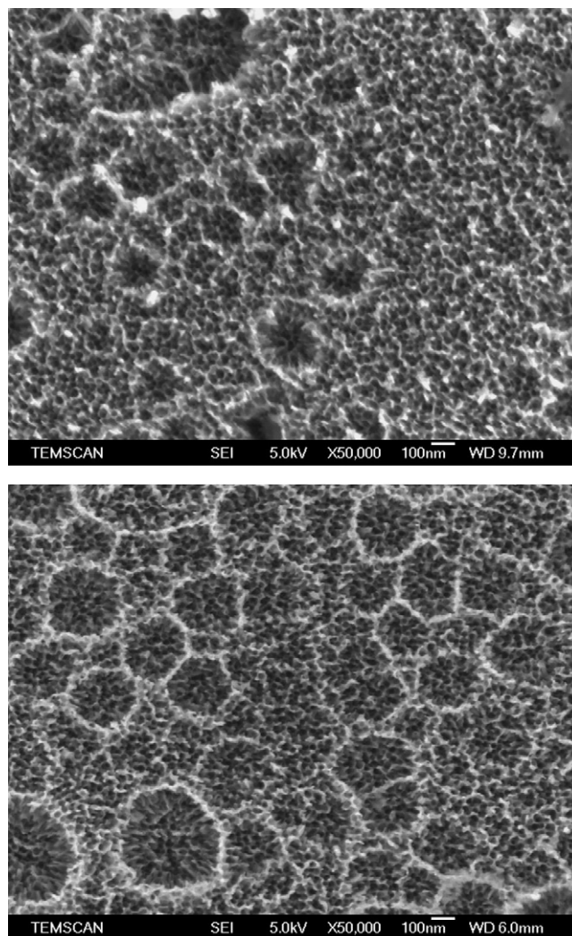
Fig. 1. FE-SEM observations of anodic films formed on Nb in 1 M \text{H}_2\text{SO}_4 + 0.2% HF (above) and 0.001 M \text{Na}_2\text{SO}_4 + 0.2% HF (below) for 1 h at 5 V.
