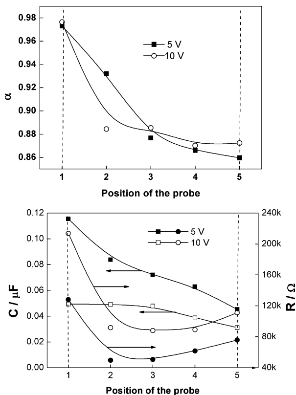
Fig. 8. CPE exponent of the high-frequency time constant (above), capacitance (left ordinate) and resistance (right ordinate) calculated from the local impedance spectra shown in Fig. 5 (below). Dashed lines indicate the boundaries of the Nb sample.
