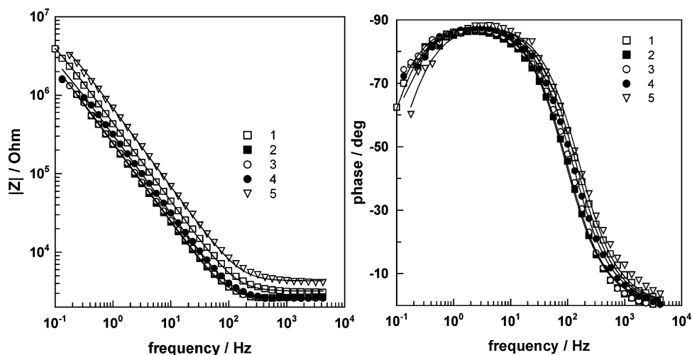
Fig. 10. Local impedance spectra of a film formed in 1 M H 2 SO 4 + 0.2% HF for 1 h at 5 V and measured at the same potential in a 0.001 M Na 2 SO 4 solution at different positions of the LEIS probe, as indicated in Fig. 5.
