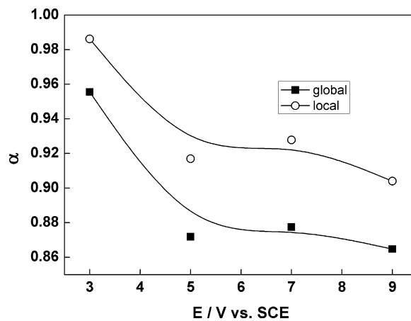
Fig. 6. CPE exponent calculated from the impedance spectra shown in Figs. 3 and 4, respectively. Global values indicated with full symbols and local values with open symbols.
