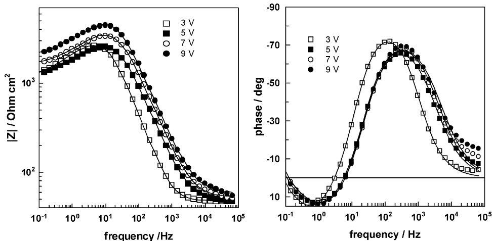
Fig. 3. Global impedance spectra for Nb in 0.001 M \text{Na}_2\text{SO}_4 + 0.2\% HF as depending on oxidation potential. Oxidation time 1 h.
