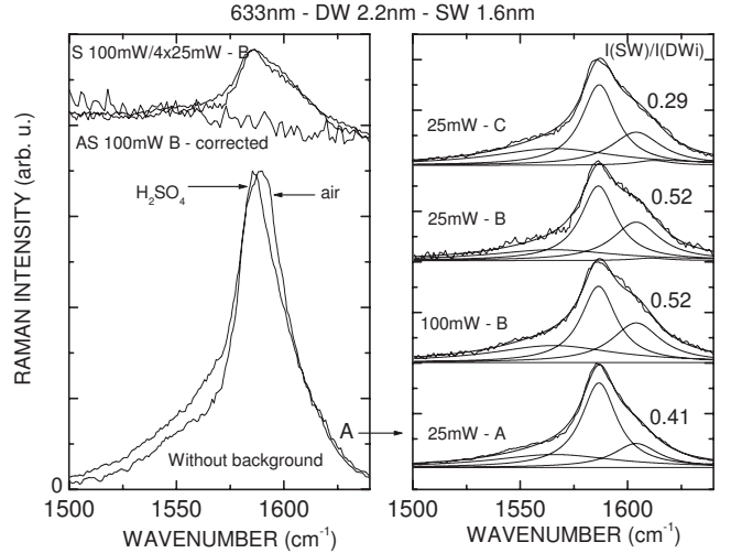
FIG. 5. Doped and undoped Raman spectra of G band of DW sample on three different locations (A, B, and C): Stokes (S) and anti-Stokes (AS) spectra after including the Bose-Einstein ( T = 775 K) and \omega^4 factors.
