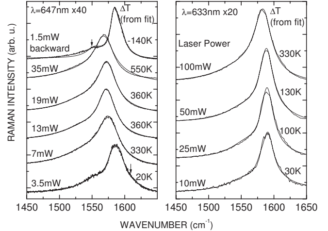
FIG. 6. DW spectra excited with red wavelengths and fitted with the parameters reported in Table III. Arrows indicate that a band at 1550 or 1610 cm -1 was used. Laser power and objective power ( \times 40 or \times 20 ) are also indicated.
