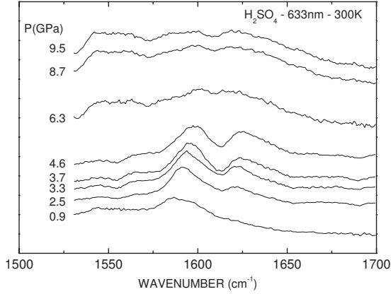
FIG. 3. G band of DW sample for pressures up to 9.5 GPa using \text{H}_2\text{SO}_4 as pressure transmitting medium.
