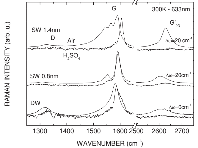
FIG. 2. Effect of doping with \text{H}_2\text{SO}_4 on Raman spectra of SW and DWs excited at 633 nm.
