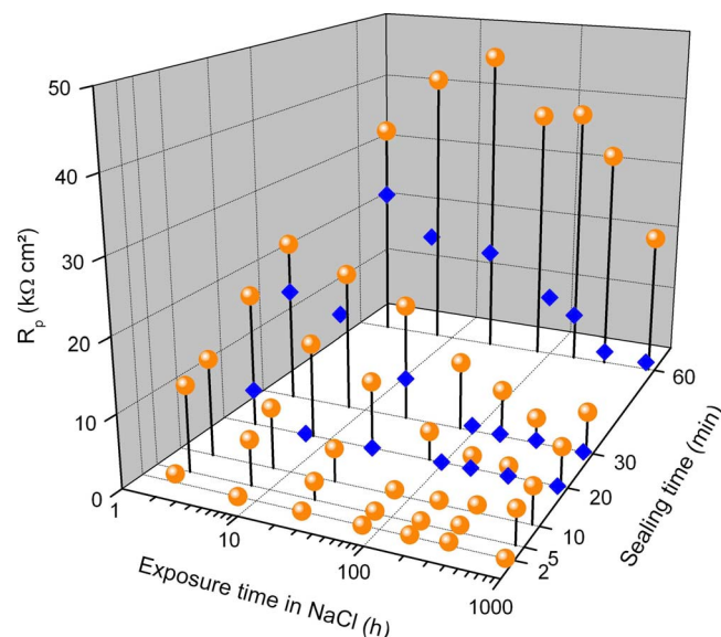
Figure 12. (Color online) R_p values for the anodic films formed in (◆) DSA and (gray circle) TSA solutions vs sealing times and vs exposure time in a 0.5 M NaCl solution.
