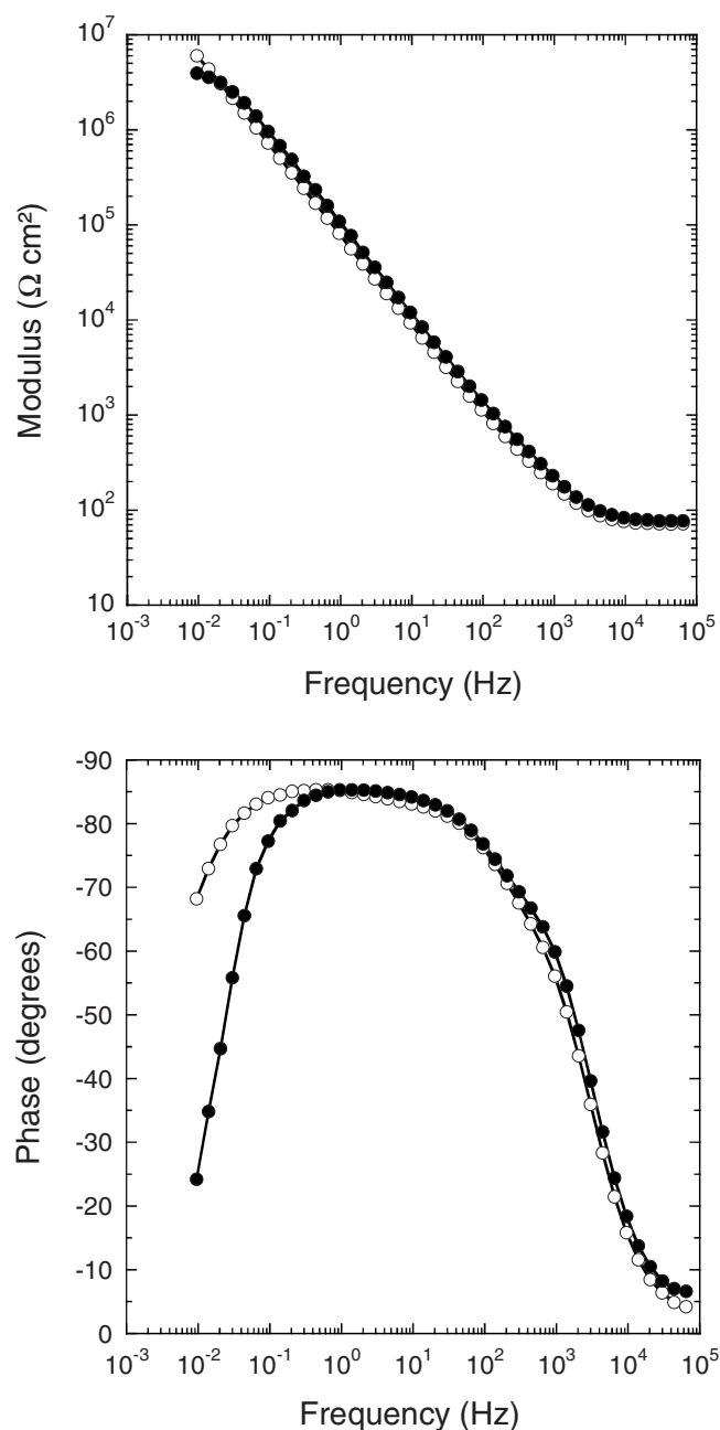
Figure 4. Bode plots of the unsealed anodic films formed in (○) DSA and in (●) TSA solutions (obtained after 2 h of immersion in 0.5 M \text{Na}_2\text{SO}_4 ).
