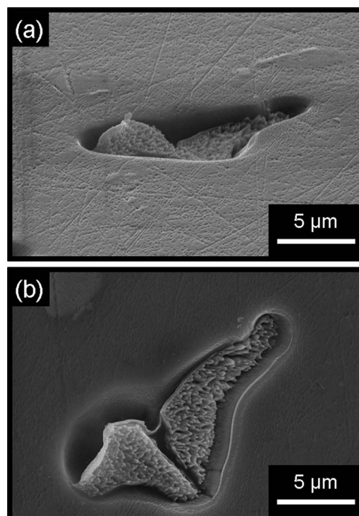
Figure 12. SEM observations of an S-phase particle in a (a) 70° tilted AA2024 specimen and (b) not tilted AA2024 specimen after immersion for 180 min in a 0.1 M \text{Na}_2\text{SO}_4 + 0.001 M NaCl solution at open-circuit potential.
