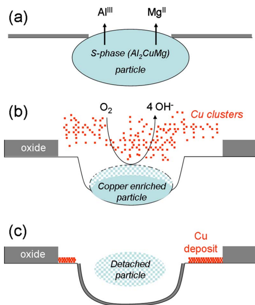
Figure 8. (Color online) Schema (not to scale) of the mechanism for the dissolution and accompanying processes occurring near an S-phase particle at open-circuit potential in a chloride-containing sulfate solution.
