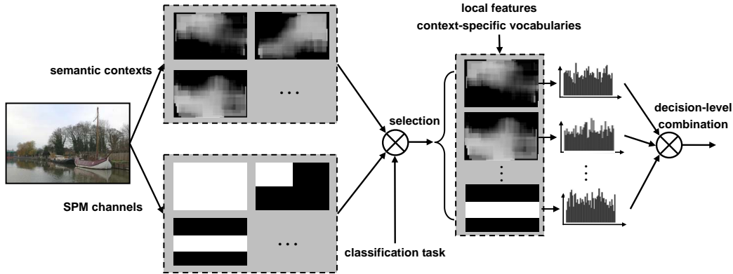
Fig. 4 Context selection from both semantic contexts and SPM channels. For an image, multiple probability maps are generated by both context classifiers and SPM channels, from which multiple BoW histograms are constructed. Then, a context selection process is used to choose a small number of the most discriminative contexts for a specific classification task. Finally, multiple BoW histograms are combined at decision level.
