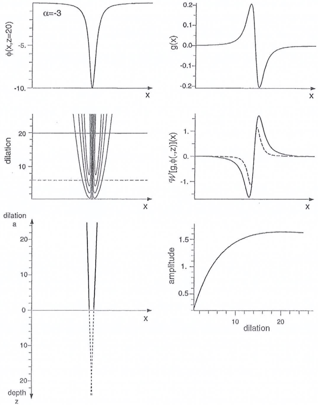
Figure 2. Wavelet analysis of the potential field measured at z = 20 and created by a homogeneous source with \alpha = -3 located at the origin (upper-left corner). Middle-left: wavelet transform of the field obtained with the analysing wavelet shown at the upper-right corner and given by equation (75). Middle-right: two voices of the wavelet transform corresponding to a = 6 (dashed curve) and a = 20 (full curve). Lower-left: the intersection of the straight lines formed by the extrema of the voices of the wavelet transform is at the source location. Lower-right: the variation of the amplitude of the wavelet transform along any line of extrema is controlled by both the depth z and the homogeneity \alpha of the source (see equations (73) and (76)).
