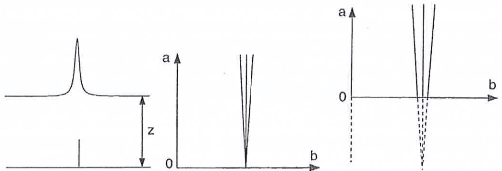
Figure 1. Wavelet transforms of singularities against wavelet transforms of potential fields. The wavelet transforms (middle) of singularities (lower left) possess lines of maxima, of zero crossings, etc, which converge on the borderline of the (b, a) half-space at the location of the singularity. The wavelet transforms (right) of potential fields (upper left) due to singular sources (e.g. point mass, lower left) and measured at a distance z possess lines of maxima, of zero crossings, etc, which converge outside the (b, a) half-space at a distance z from the borderline. This property is satisfied only for a particular class of analysing wavelets introduced in this paper.
