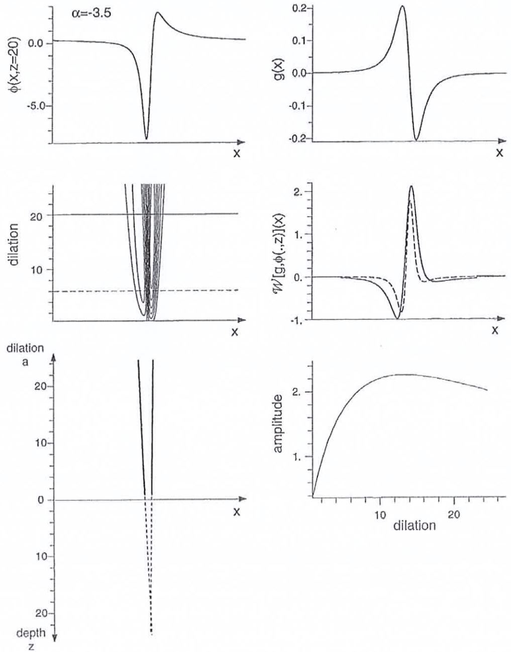
Figure 3. Same as figure 2 for \alpha = -3.5 .
