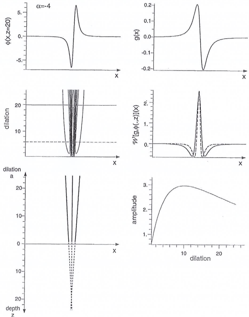
Figure 4. Same as figure 2 for \alpha = -4 .
