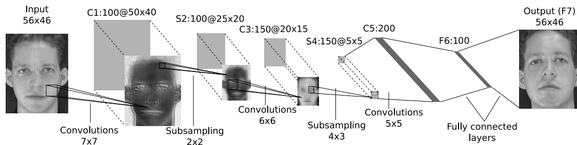
Figure 2. Architecture of the Network.
