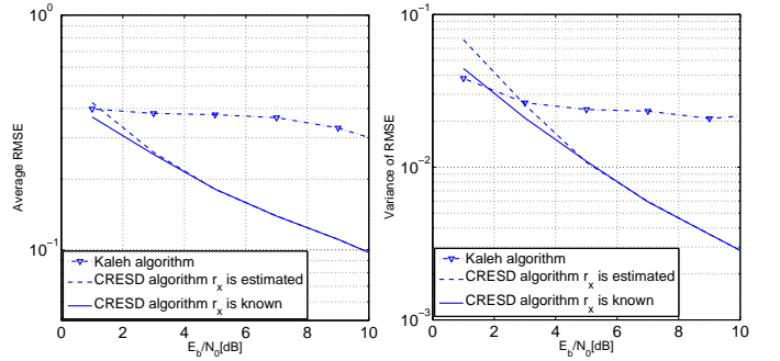
Fig. 3: RMSE vs E_b/N_0 , for N=100 , L=3 and r_x = 3
