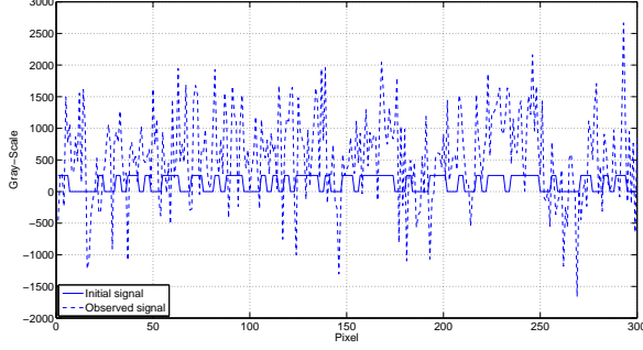
Fig. 2: Blurred signal with blur length L=10 , r_x = 3 and N = 100
