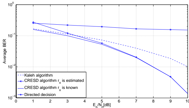
Fig. 5: BER performance for known and estimated r_x , L=3 , r_x = 3 , N = 100
