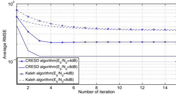
Fig. 4: Evolution of the RMSE with iterations, with L = 3 , r_x = 3 and N = 100
