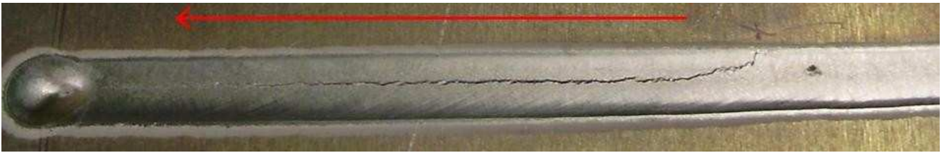
Figure 2: Autogenous weld bead and crack location.
