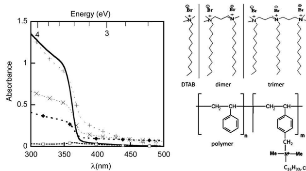
Fig. 2 Absorbance measurements of the aqueous phases after the transfer procedure using the various surfactants compared to the absorbance of the pristine NCs in the organic solution before transfer. (—) Before transfer; (□) monomer = DTAB; (◆) dimer; (×) trimer; (+) polymer. Surfactant concentration: 2 mM.
