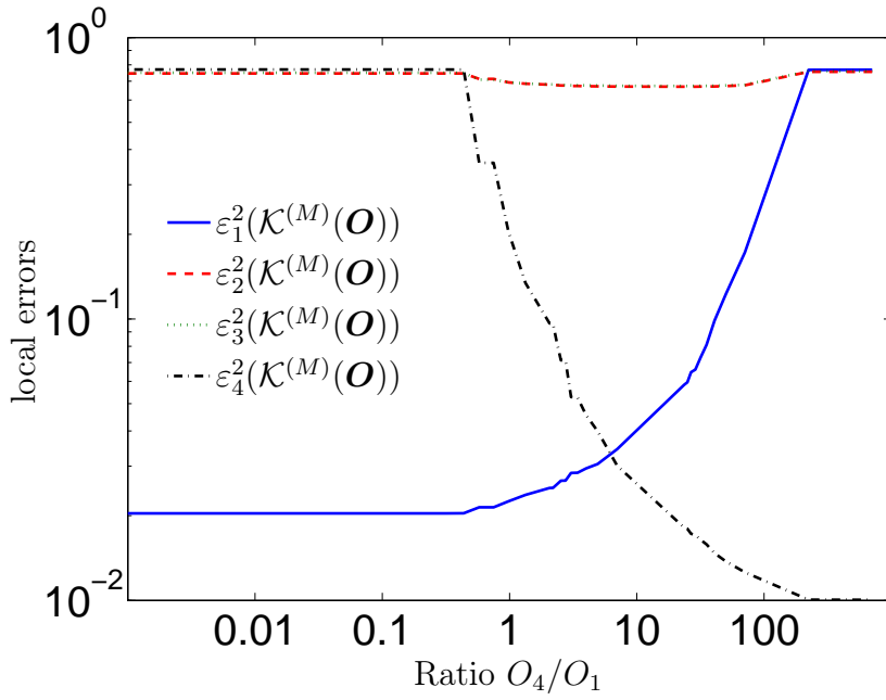
Figure 5: Comparison of local errors \varepsilon_q^2(\mathcal{K}^{(M)}(\mathbf{O})) , when \mathbf{O} = \frac{1}{\sqrt{O_1^2 + 2 \cdot 10^{-10} + O_4^2}}(O_1, 10^{-5}, 10^{-5}, O_4) with respect to ratio O_4/O_1 , for M = 50 .
