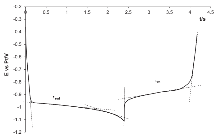
Fig. 4. Reversed chronopotentiogram of the LiF–CaF 2 –ZrF 4 (0.08 mol kg -1 ) system at 840 °C; applied current = ±0.15 A. Working el.: Ta ( S=0.31 cm 2 ); auxiliary el.: glassy carbon; comparison el.: Pt.
