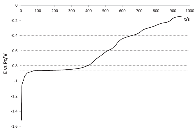
Fig. 11. Open-circuit chronopotentiogram of glassy LiF-CaF_2-ZrF_4 ( 0.11 \text{ mol kg}^{-1} ) on Cu electrode ( S=0.31 \text{ cm}^2 ) at 840^\circ C after a polarization at I=-0.2 \text{ A} . Auxiliary el.: glassy carbon; comparison el.: Pt.
