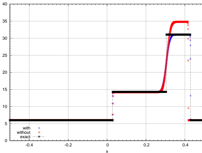
FIGURE 2. Test 5 of [63, chapter 4] - Density obtained with n = 2000 cells, with and without corrective source terms, and analytical solution.
