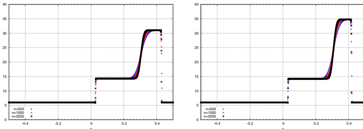
FIGURE 3. Test 5 of [63, chapter 4] - Density obtained with various meshes, with (left) and without (right) corrective source terms.
