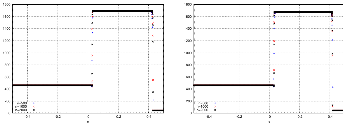
FIGURE 4. Test 5 of [63, chapter 4] - pressure obtained with various meshes, with (left) and without (right) corrective source terms.
