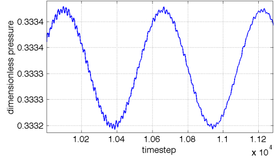
Figure 7: Pressure calculated at the pipe's inlet section.
