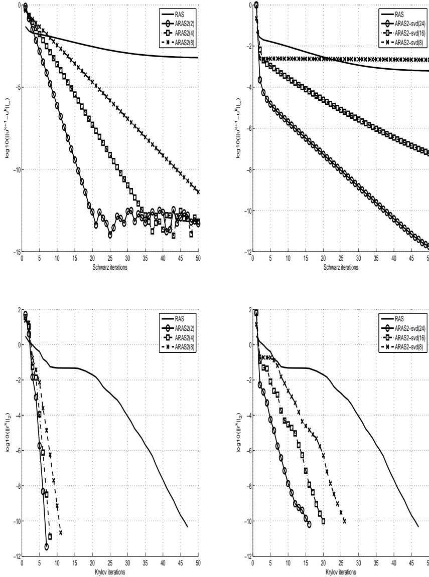
FIGURE 5.3. Solving 2D Helmholtz equation on a 164 \times 164 Cartesian grid, physical band partitioning, p = 8 , (left) ARAS2( r = \frac{p}{q} ) is built with a Random base, (right) ARAS2( q ) is built with a SVD base, (top) Convergence of Iterative Schwarz Process, (bottom) convergence of GCR method preconditioned by RAS and ARAS2.
